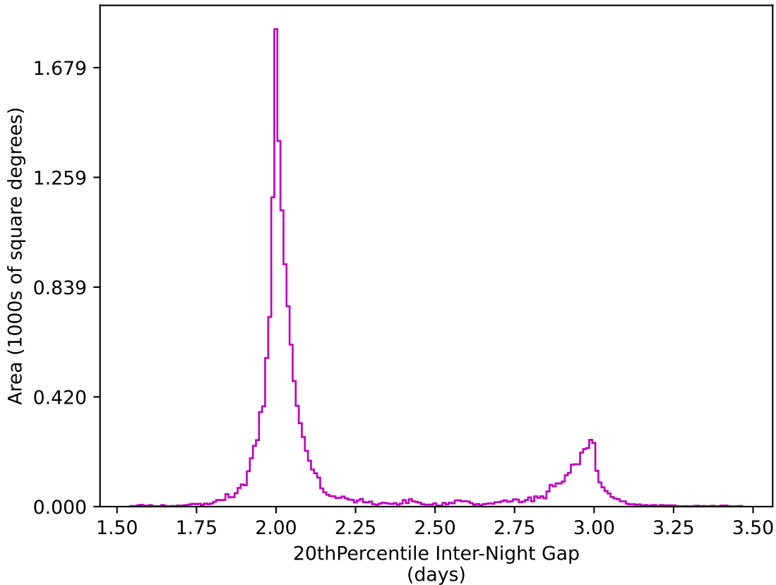
ddf_loaded_half_fl2_v3.4_10yrs WFD z band: 20thPercentile Inter-Night Gap
