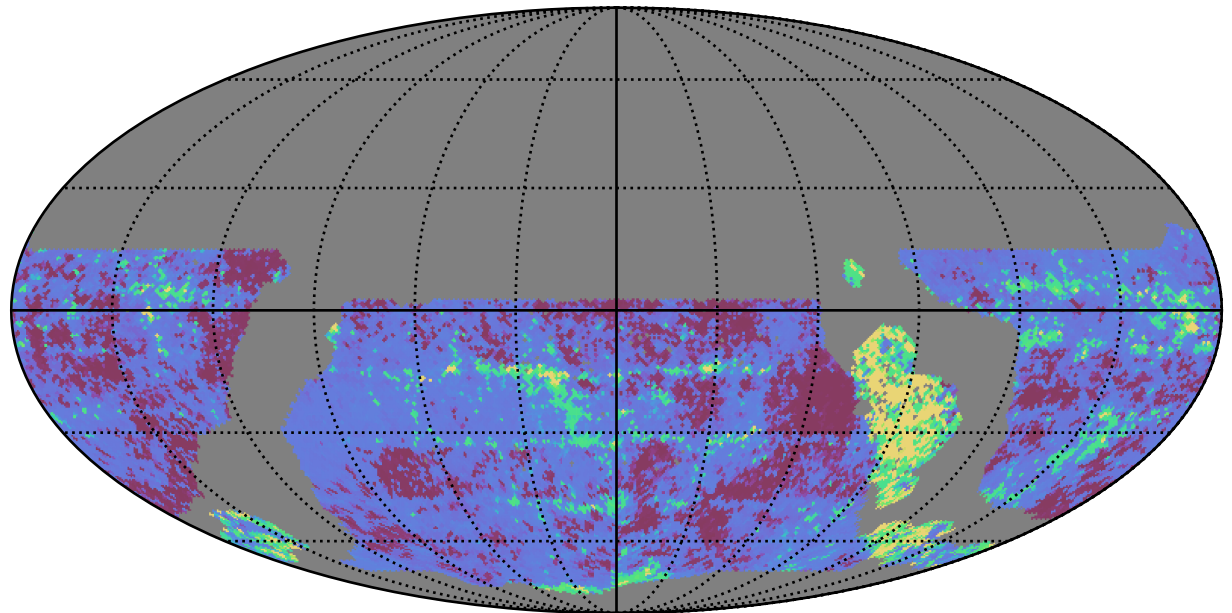
ddf_loaded_half_fl2_v3.4_10yrs WFD y band: 20thPercentile Inter-Night Gap
