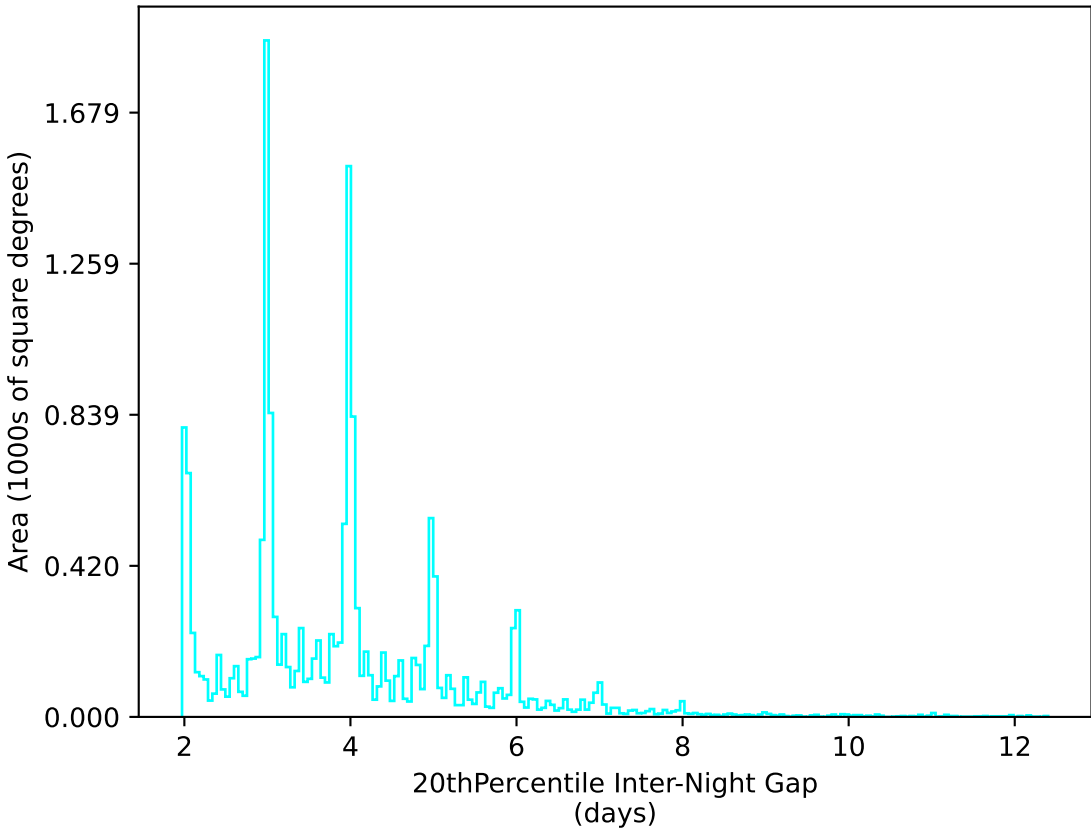
ddf_loaded_half_fl2_v3.4_10yrs WFD u band: 20thPercentile Inter-Night Gap
