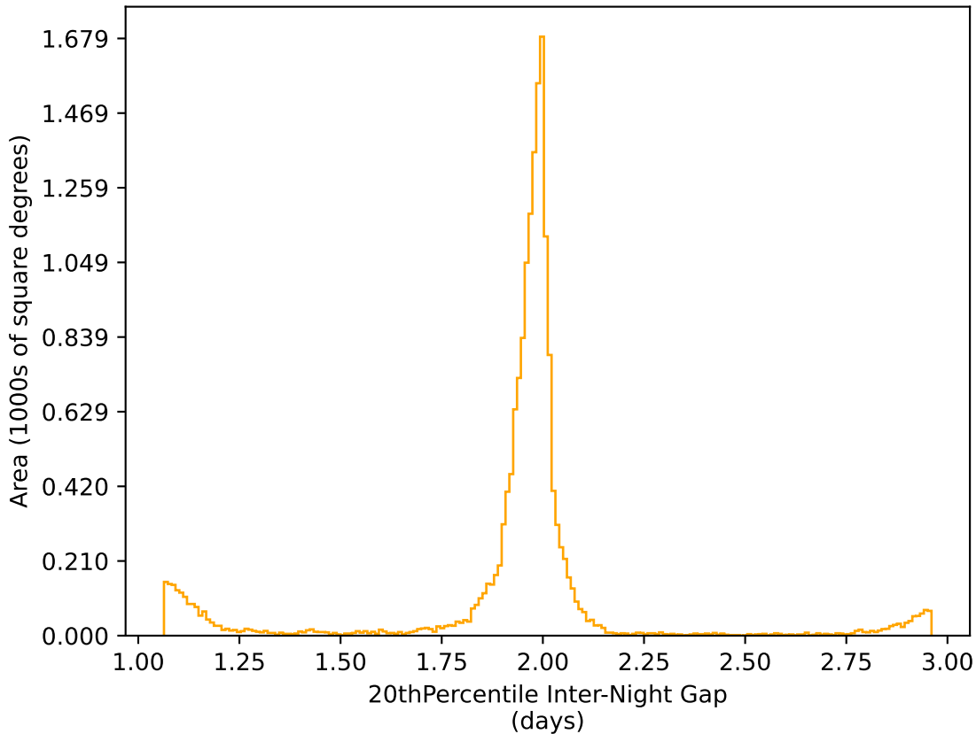
ddf_loaded_half_fl2_v3.4_10yrs WFD r band: 20thPercentile Inter-Night Gap
