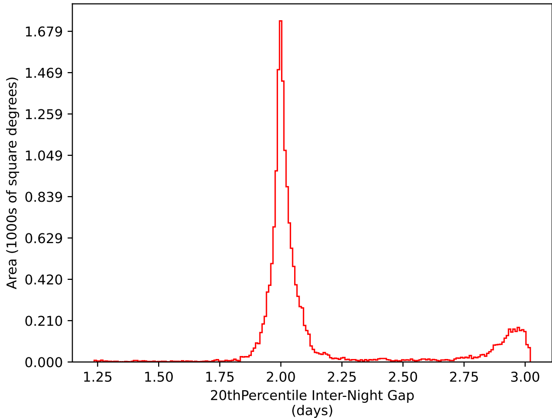
ddf_loaded_half_fl2_v3.4_10yrs WFD i band: 20thPercentile Inter-Night Gap
