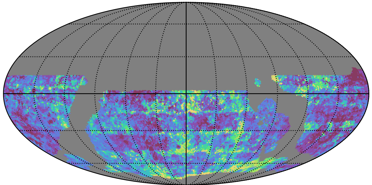
ddf_loaded_half_fl2_v3.4_10yrs WFD g band: 20thPercentile Inter-Night Gap
