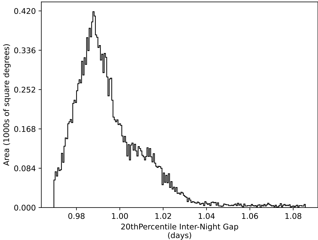
ddf_loaded_half_fl2_v3.4_10yrs WFD all bands: 20thPercentile Inter-Night Gap
