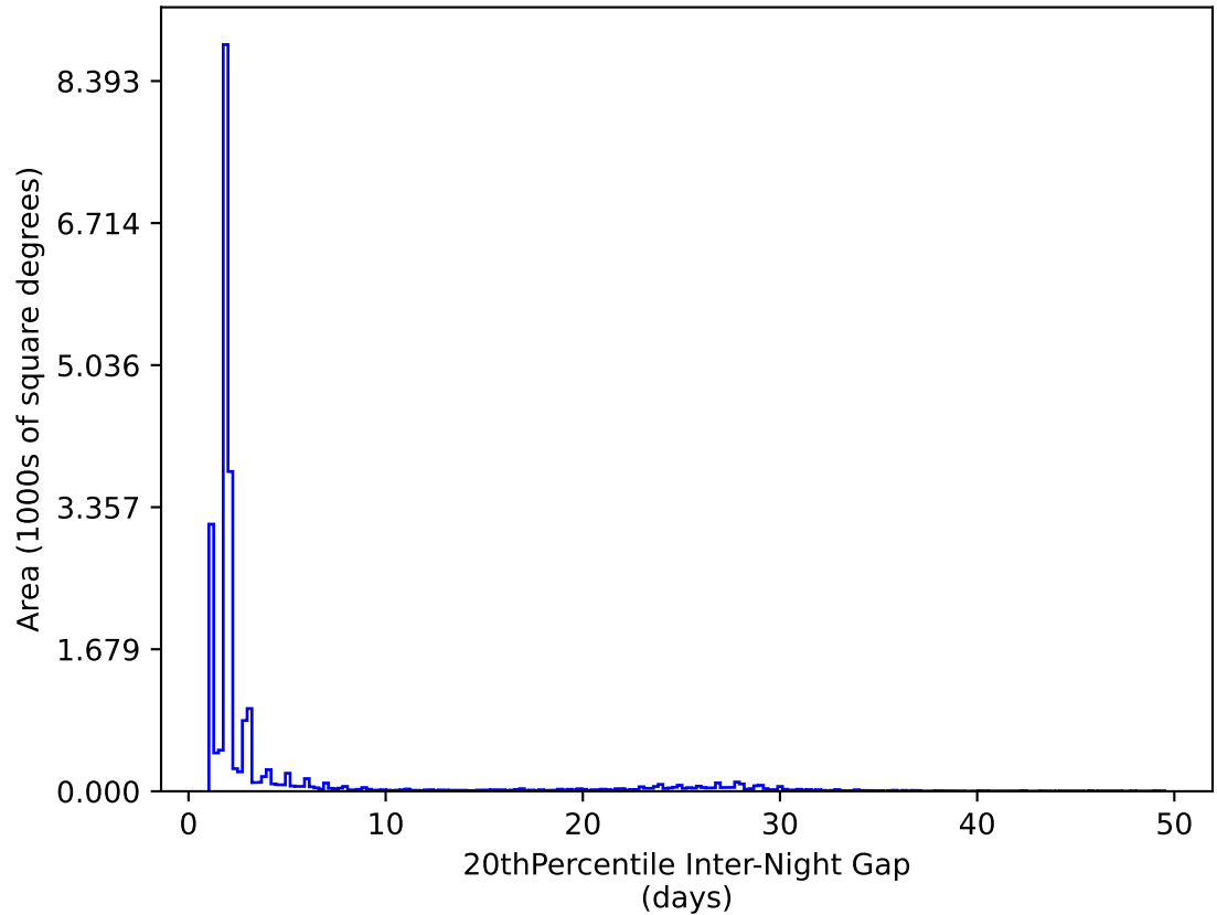
ddf_loaded_half_fl2_v3.4_10yrs All sky y band: 20thPercentile Inter-Night Gap
