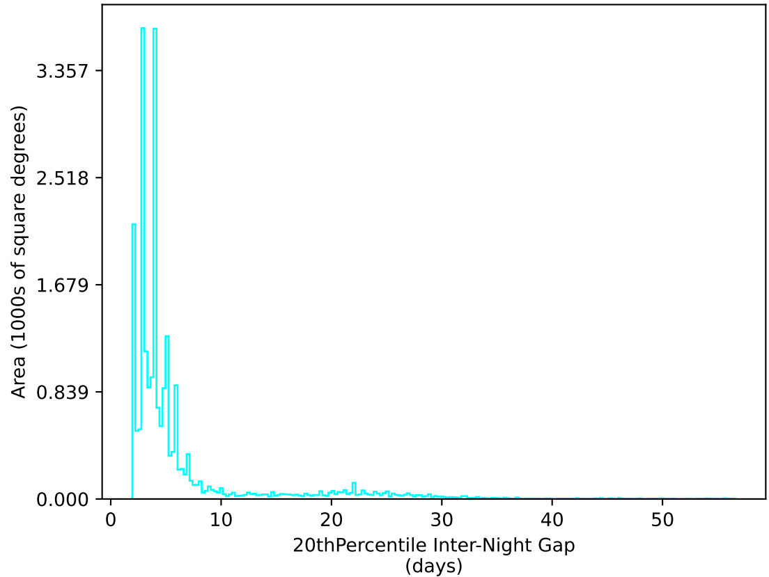
ddf_loaded_half_fl2_v3.4_10yrs All sky u band: 20thPercentile Inter-Night Gap
