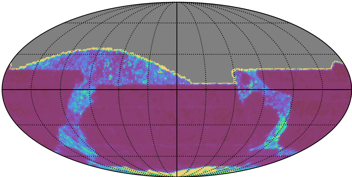
ddf_loaded_half_fl2_v3.4_10yrs All sky r band: 20thPercentile Inter-Night Gap
