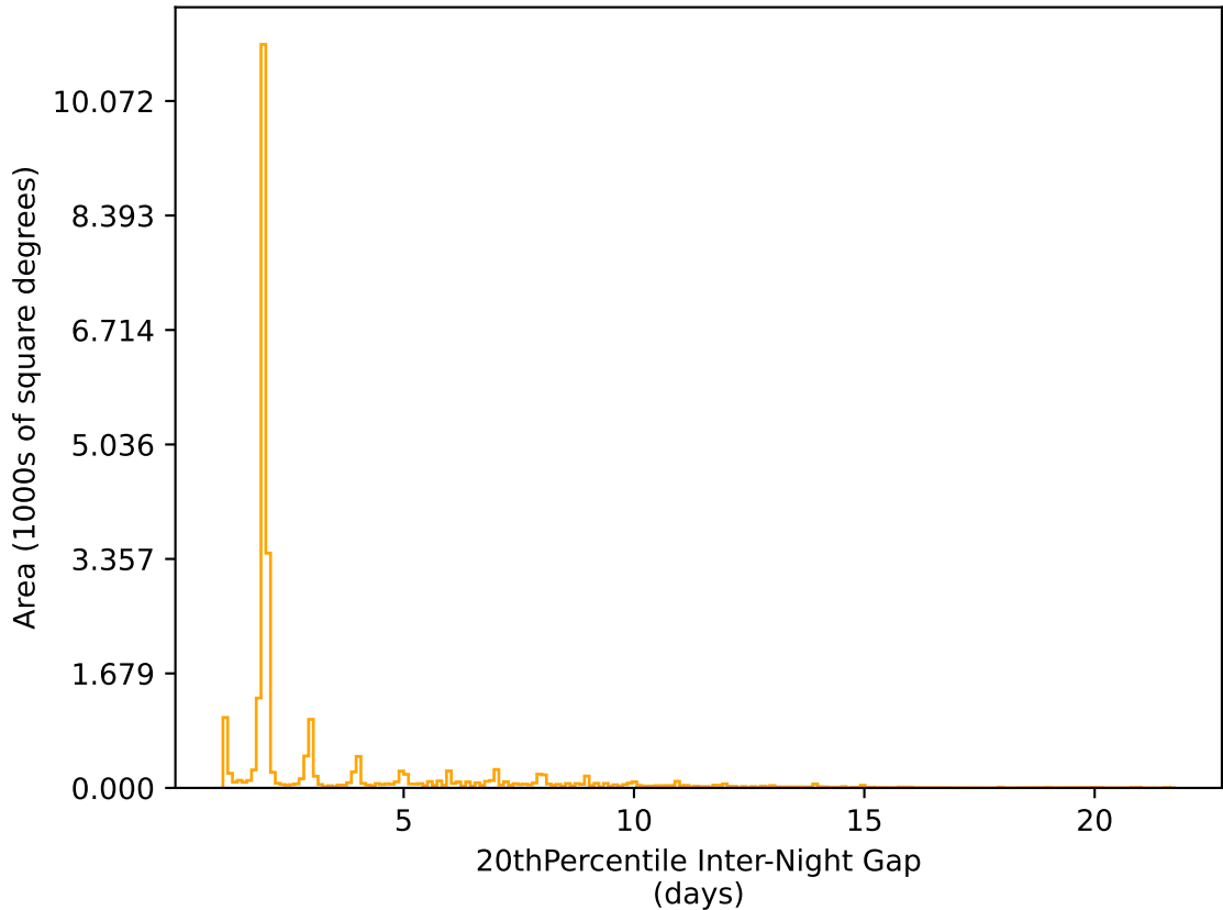
ddf_loaded_half_fl2_v3.4_10yrs All sky r band: 20thPercentile Inter-Night Gap
