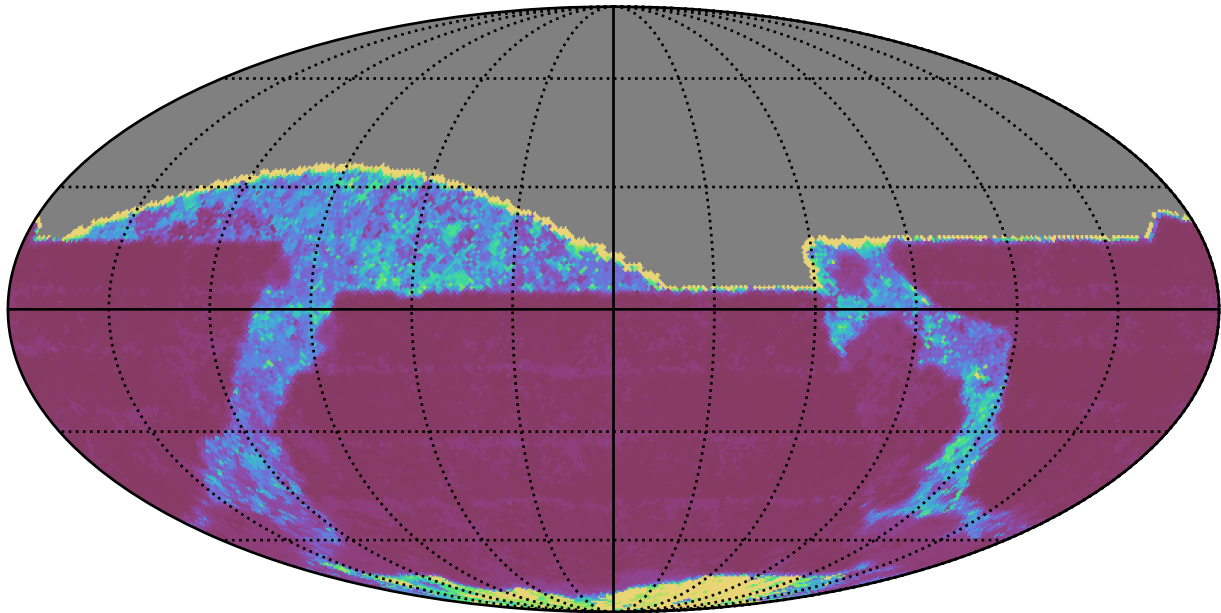
ddf_loaded_half_fl2_v3.4_10yrs All sky i band: 20thPercentile Inter-Night Gap
