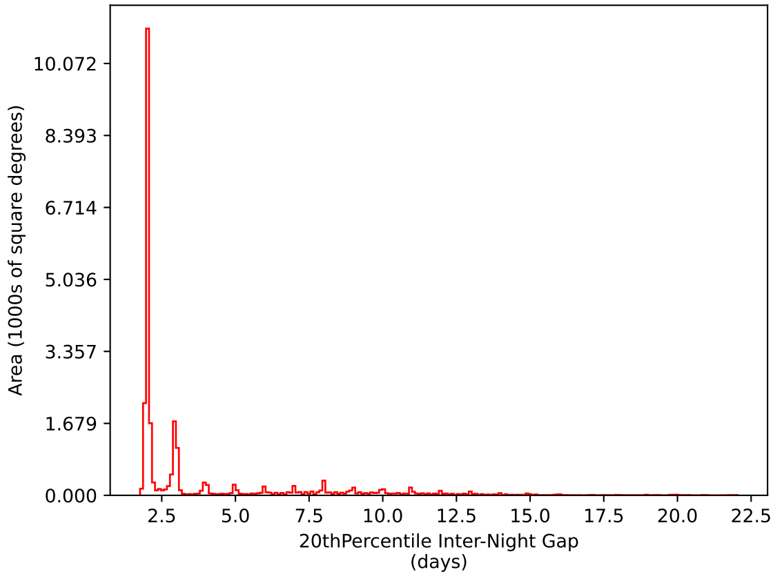
ddf_loaded_half_fl2_v3.4_10yrs All sky i band: 20thPercentile Inter-Night Gap
