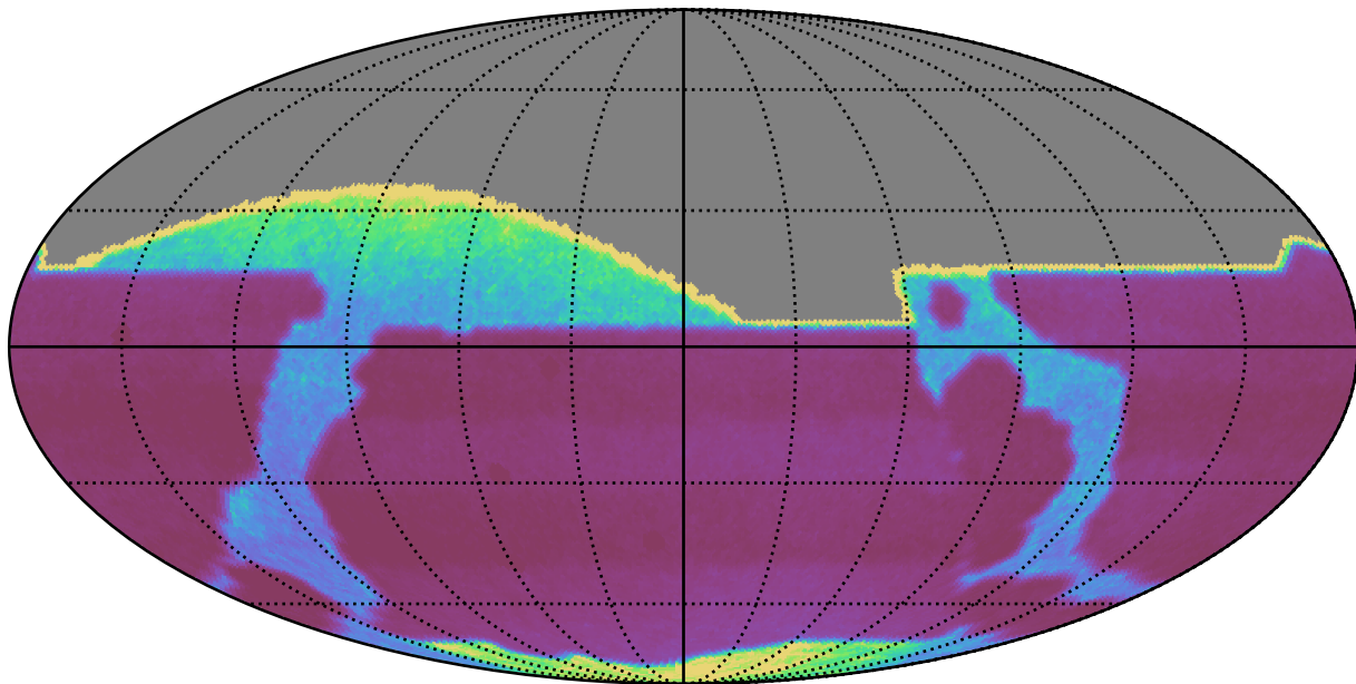
ddf_loaded_half_fl2_v3.4_10yrs : properMotion
