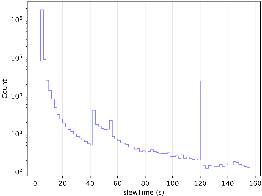
ddf_loaded_half_fl2_v3.4_10yrs All visits: Slew Time Histogram
