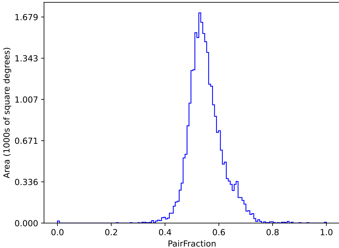
ddf_loaded_half_fl2_v3.4_10yrs (g or r or i): PairFraction
