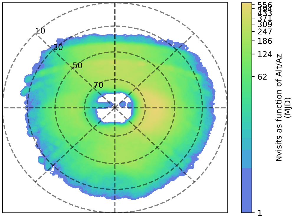
ddf_loaded_half_fl2_v3.4_10yrs u: Nvisits as function of Alt/Az
