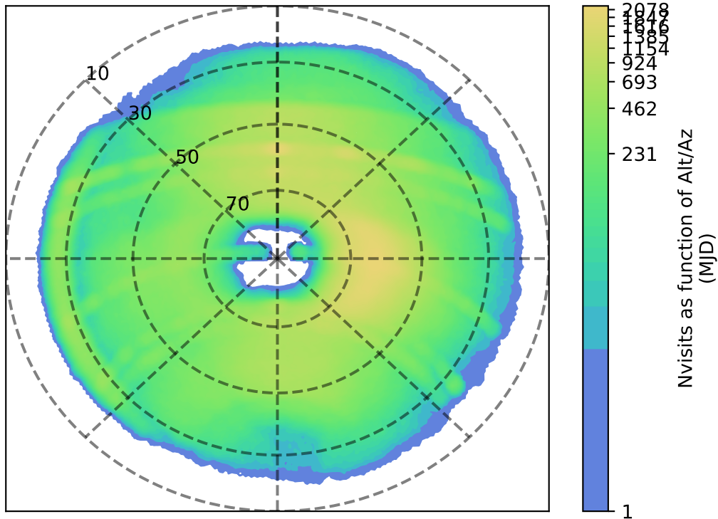
ddf_loaded_half_fl2_v3.4_10yrs r: Nvisits as function of Alt/Az
