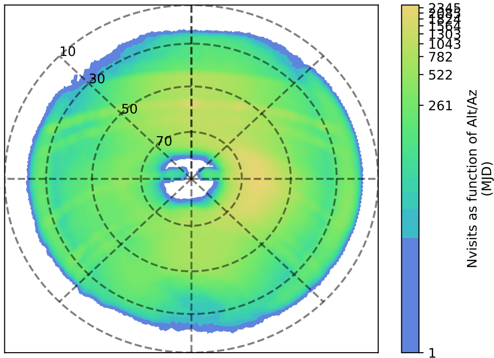
ddf_loaded_half_fl2_v3.4_10yrs i: Nvisits as function of Alt/Az
