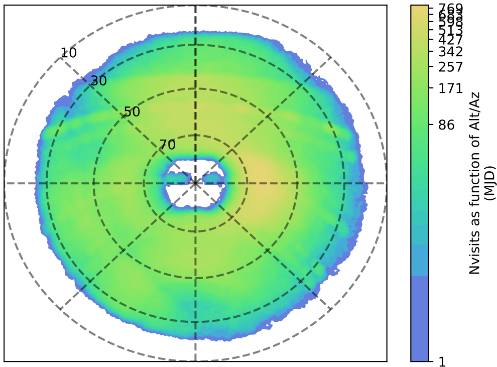
ddf_loaded_half_fl2_v3.4_10yrs g: Nvisits as function of Alt/Az
