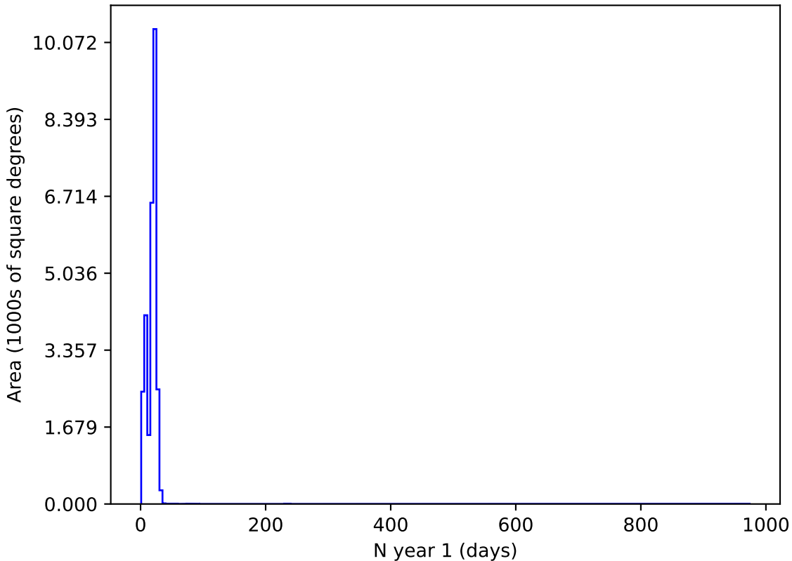
ddf_loaded_half_fl2_v3.4_10yrs i and night < 365: N year 1
