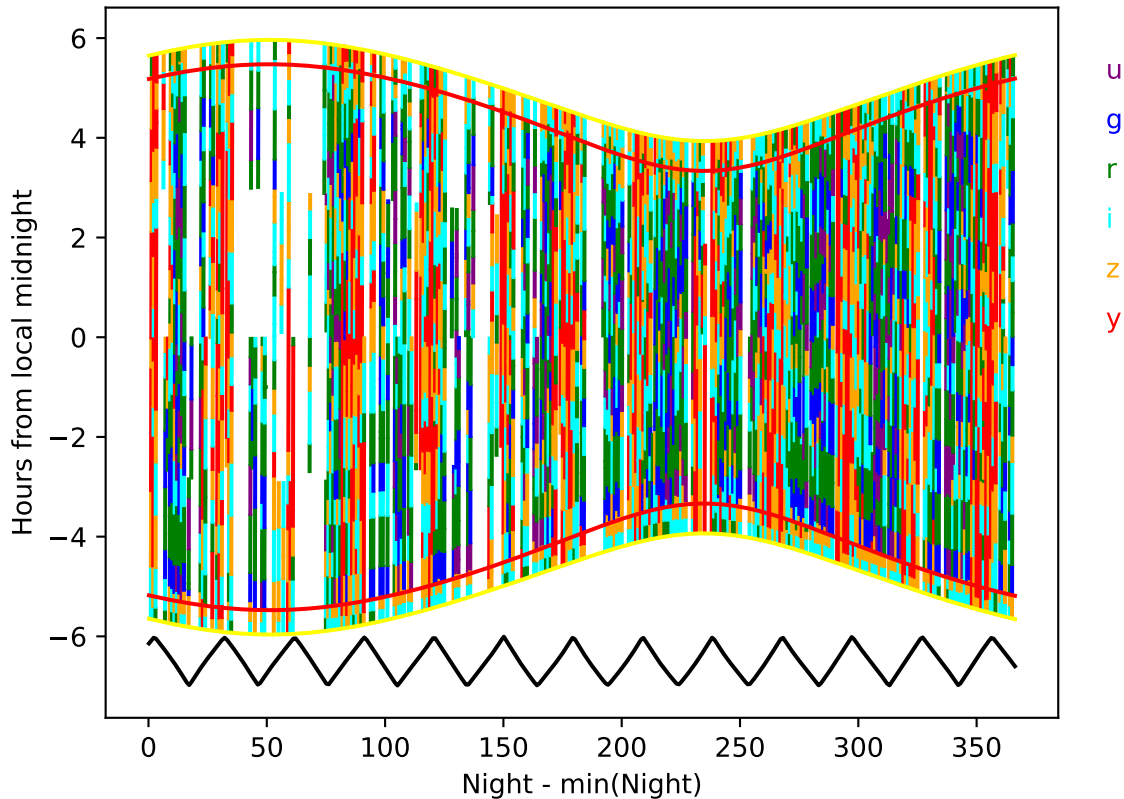
ddf_loaded_half_fl2_v3.4_10yrs year 9-10: Hourglass
