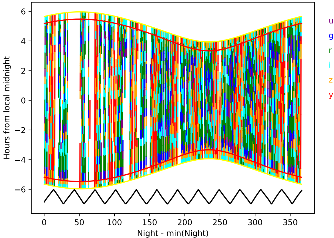
ddf_loaded_half_fl2_v3.4_10yrs year 8-9: Hourglass
