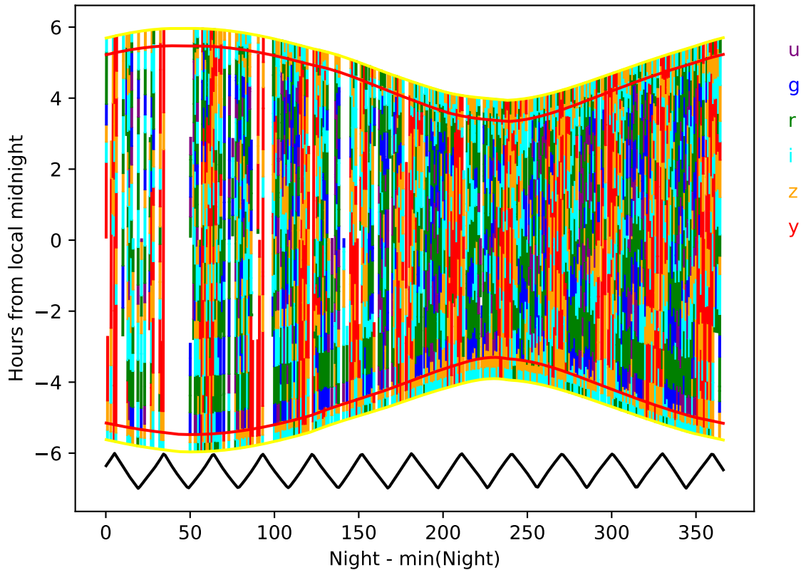
ddf_loaded_half_fl2_v3.4_10yrs year 6-7: Hourglass
