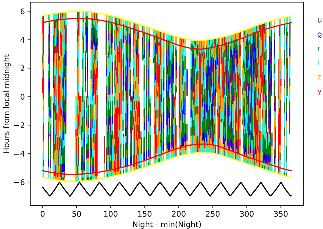
ddf_loaded_half_fl2_v3.4_10yrs year 4-5: Hourglass
