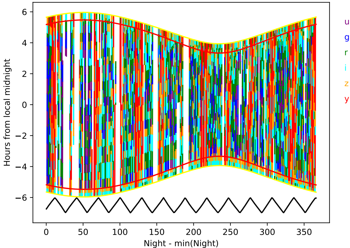
ddf_loaded_half_fl2_v3.4_10yrs year 0-1: Hourglass
