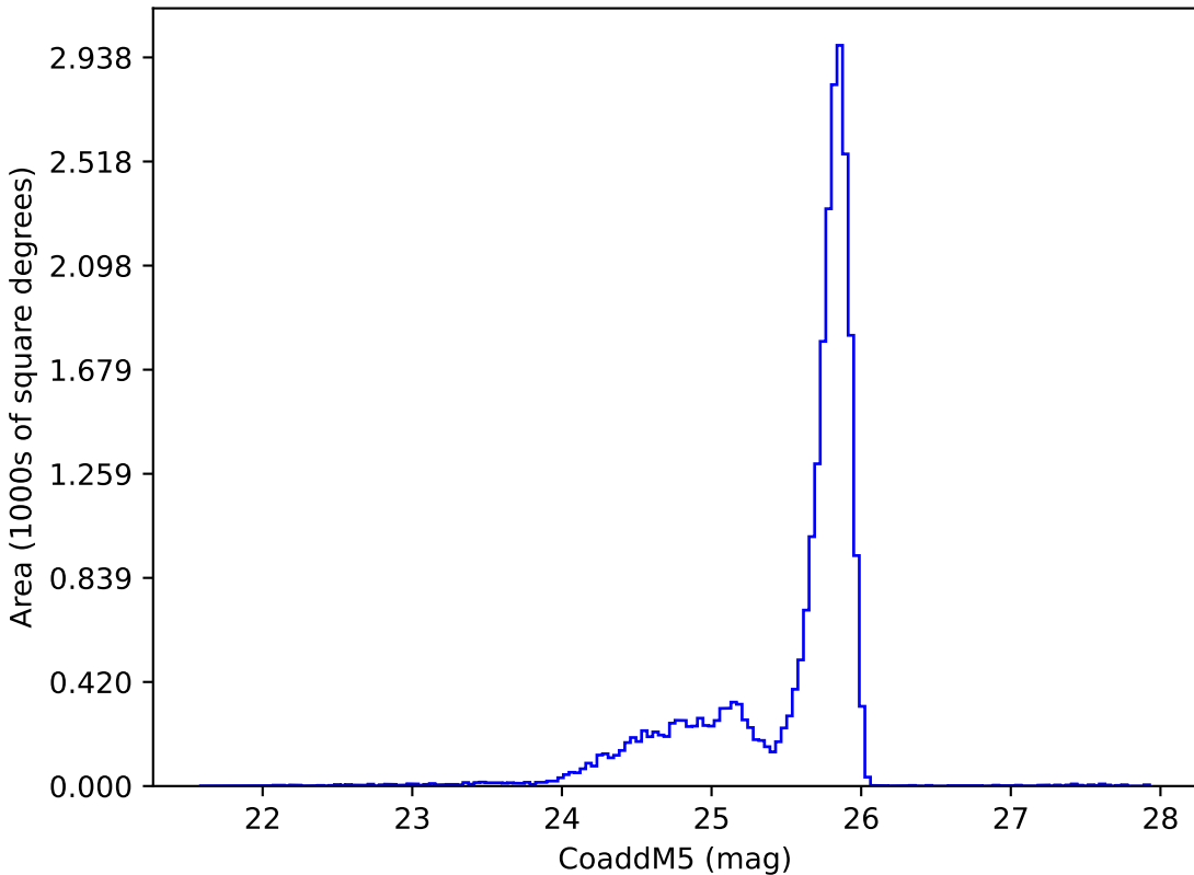
ddf_loaded_half_fl2_v3.4_10yrs z: CoaddM5
