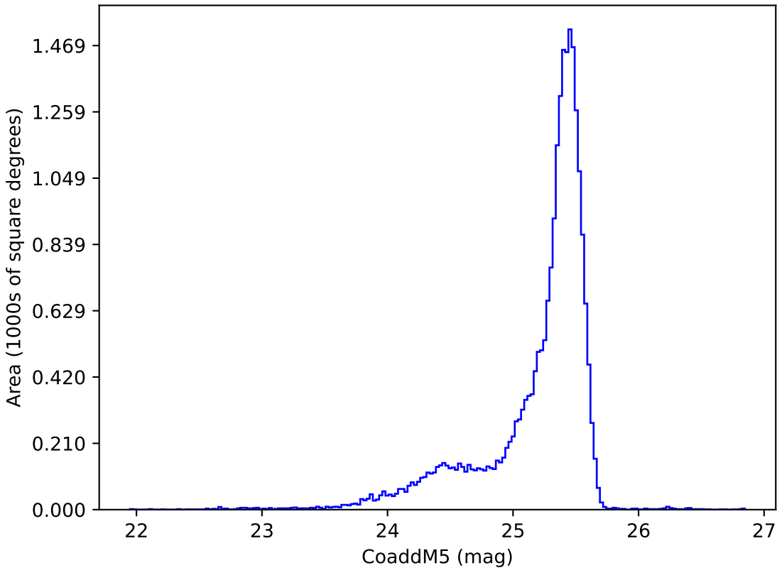
ddf_loaded_half_fl2_v3.4_10yrs u: CoaddM5
