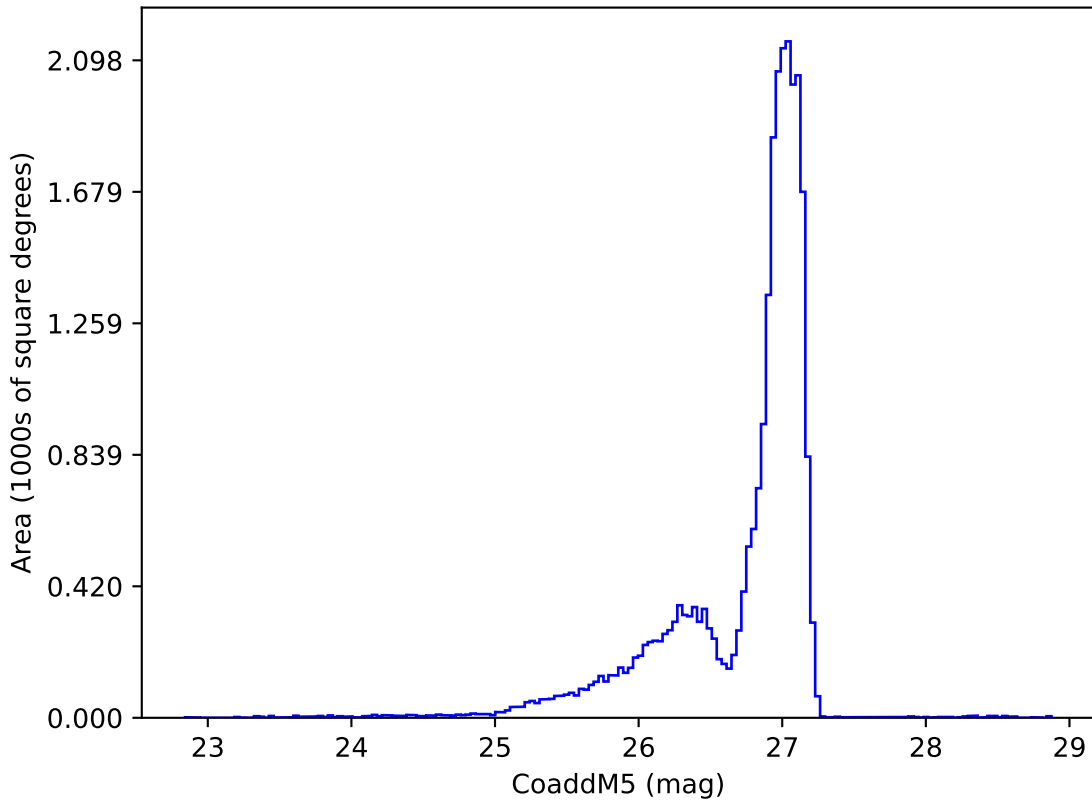
ddf_loaded_half_f12_v3.4_10yrs r: CoaddM5
