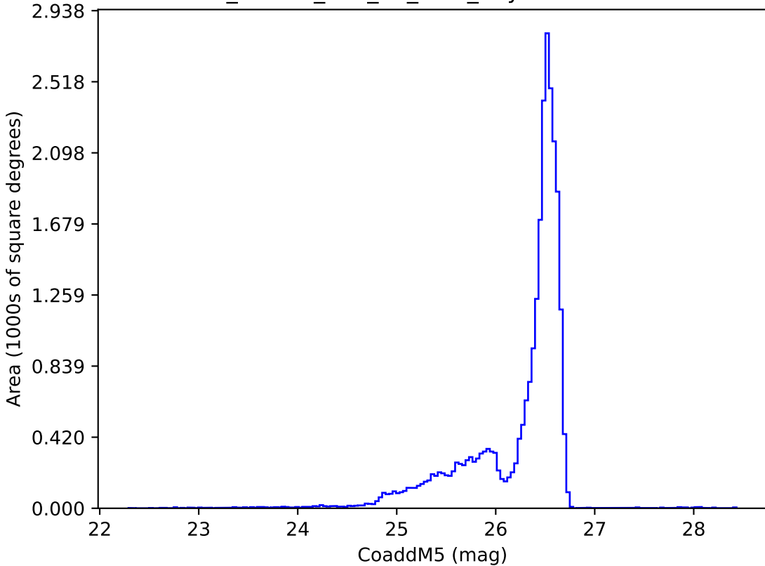
ddf_loaded_half_fl2_v3.4_10yrs i: CoaddM5
