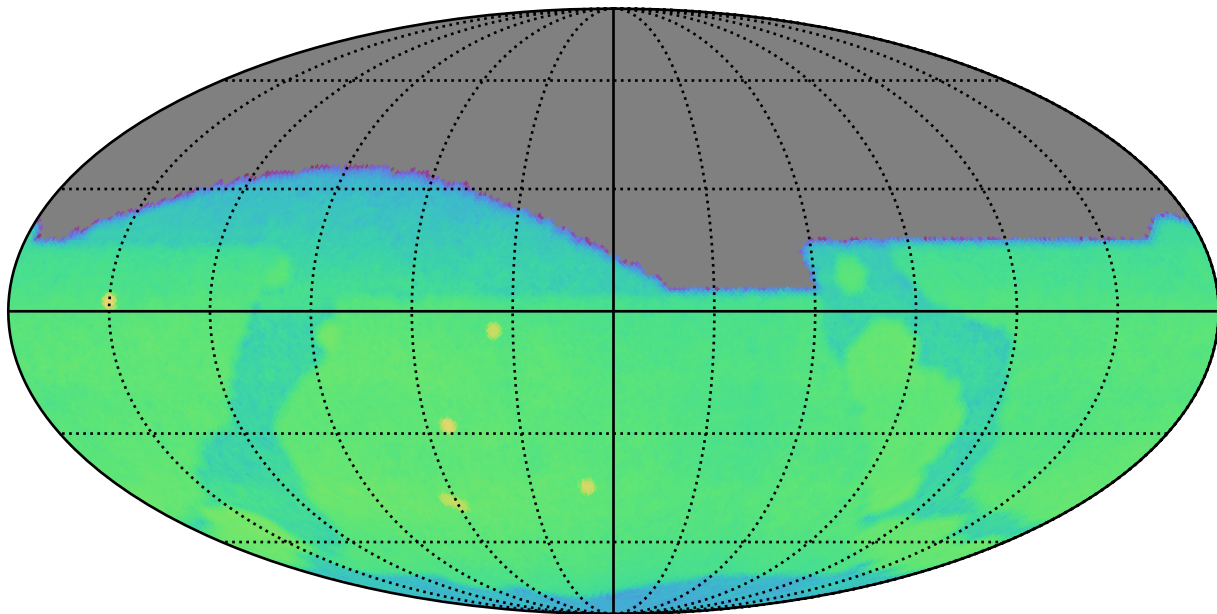
ddf_loaded_half_f12_v3.4_10yrs g: CoaddM5
