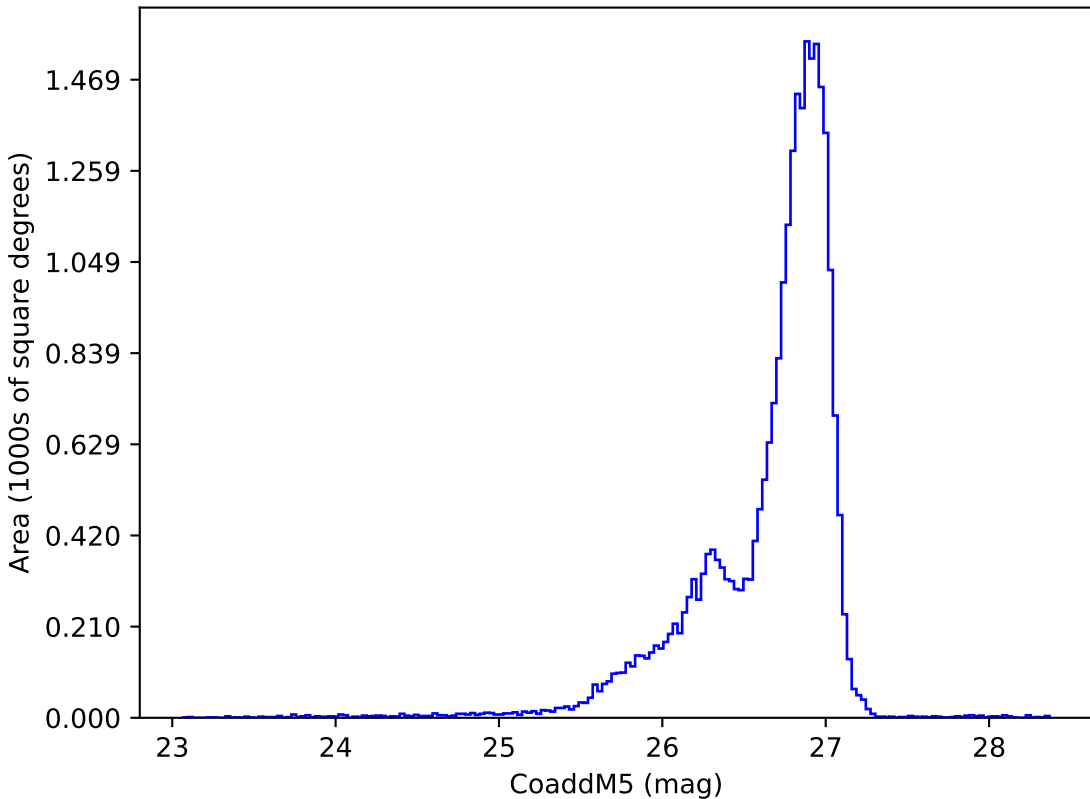
ddf_loaded_half_fl2_v3.4_10yrs g: CoaddM5
