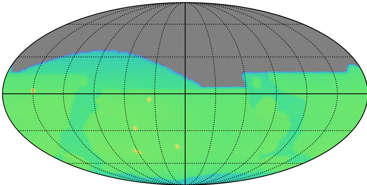
ddf_loaded_half_fl2_v3.4_10yrs : CoaddM5
