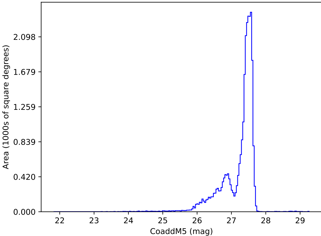
ddf_loaded_half_fl2_v3.4_10yrs : CoaddM5
