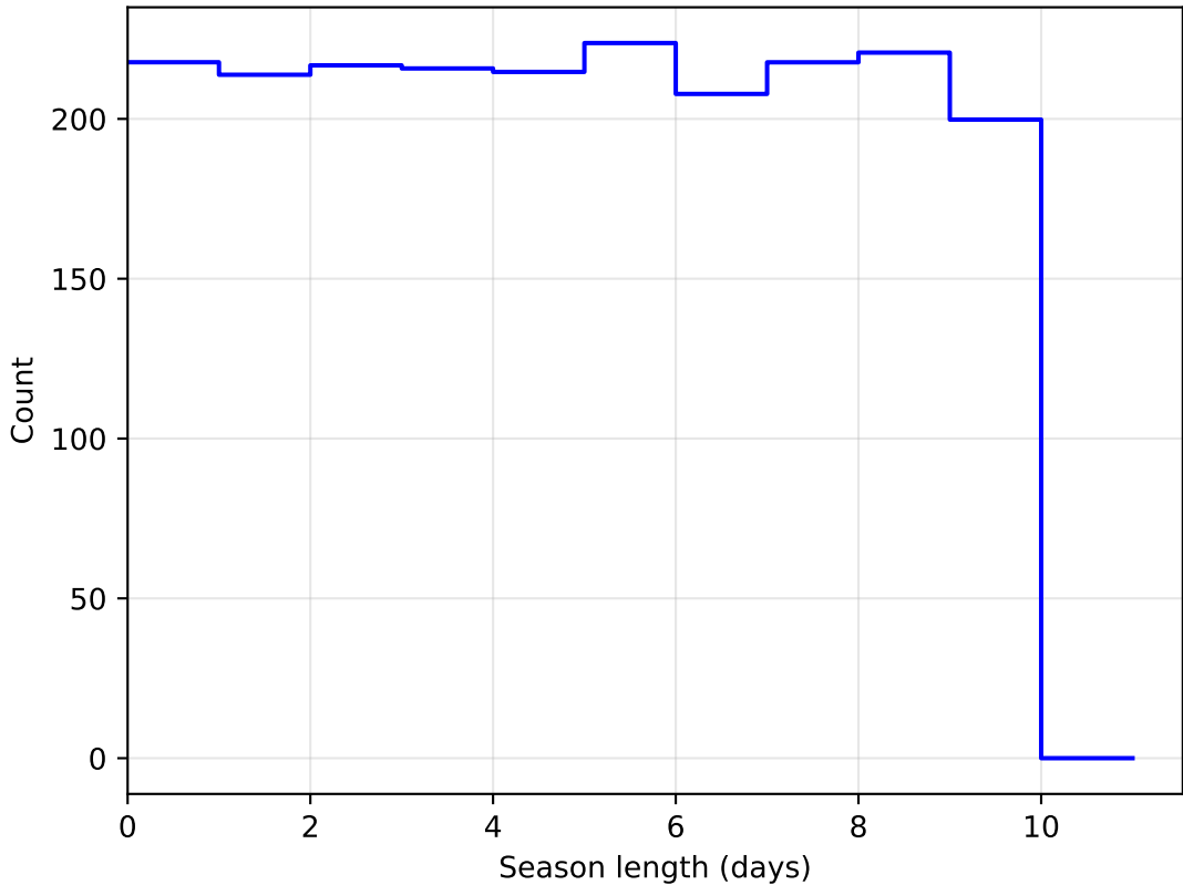
ddf_loaded_half_fl2_v3.4_10yrs DD:ECDFS all bands: SeasonLength
