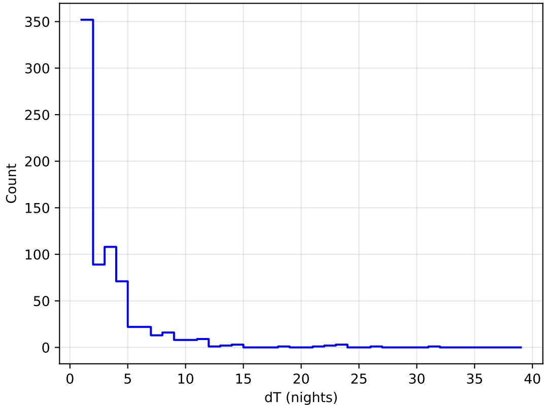
ddf_loaded_half_fl2_v3.4_10yrs all bands: DD:XMM_LSS Delta Nights Histogram
