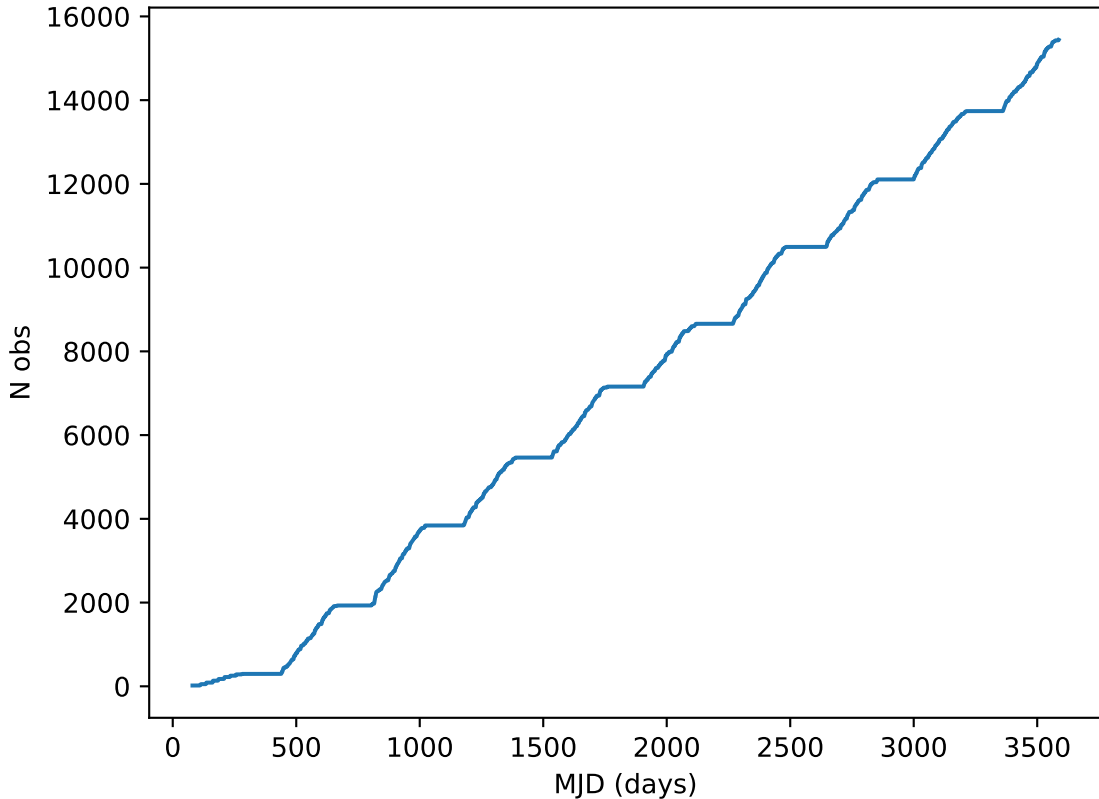
ddf_loaded_half_fl2_v3.4_10yrs all bands: DD:XMM_LSS Cumulative NVisits
