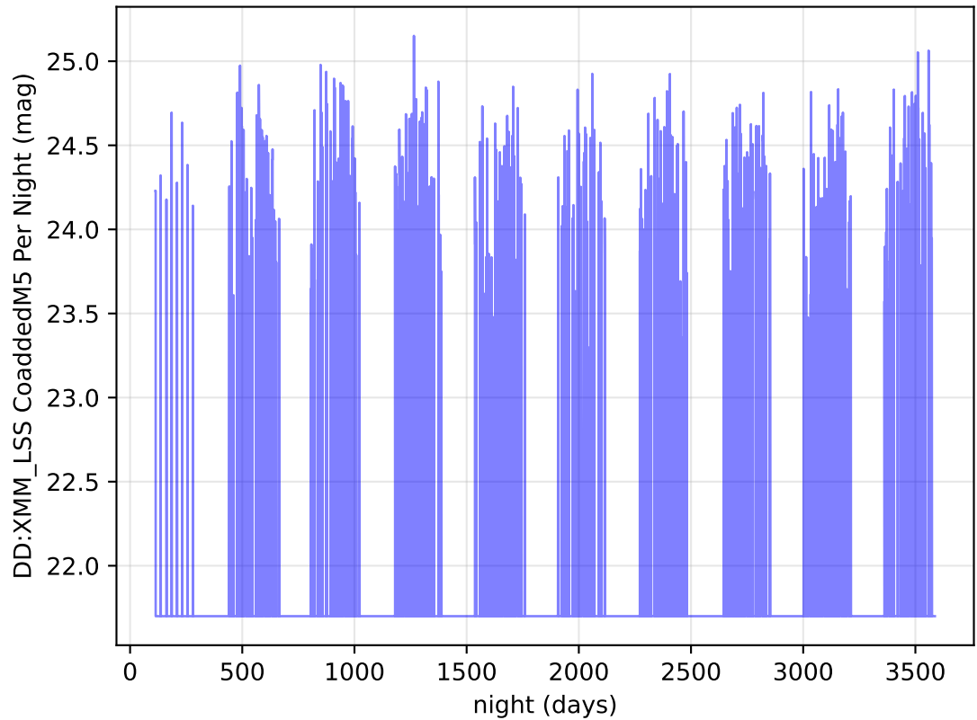
ddf_loaded_half_fl2_v3.4_10yrs z band: DD:XMM_LSS CoaddedM5 Per Night
