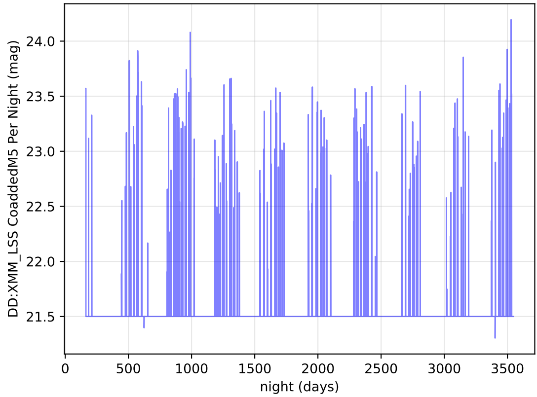
ddf_loaded_half_fl2_v3.4_10yrs y band: DD:XMM_LSS CoaddedM5 Per Night
