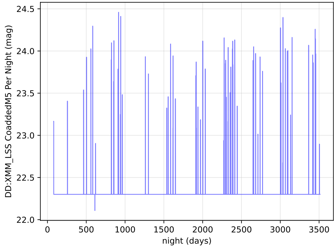
ddf_loaded_half_fl2_v3.4_10yrs u band: DD:XMM_LSS CoaddedM5 Per Night
