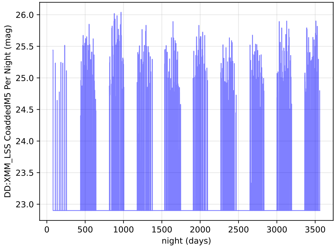
ddf_loaded_half_fl2_v3.4_10yrs r band: DD:XMM_LSS CoaddedM5 Per Night
