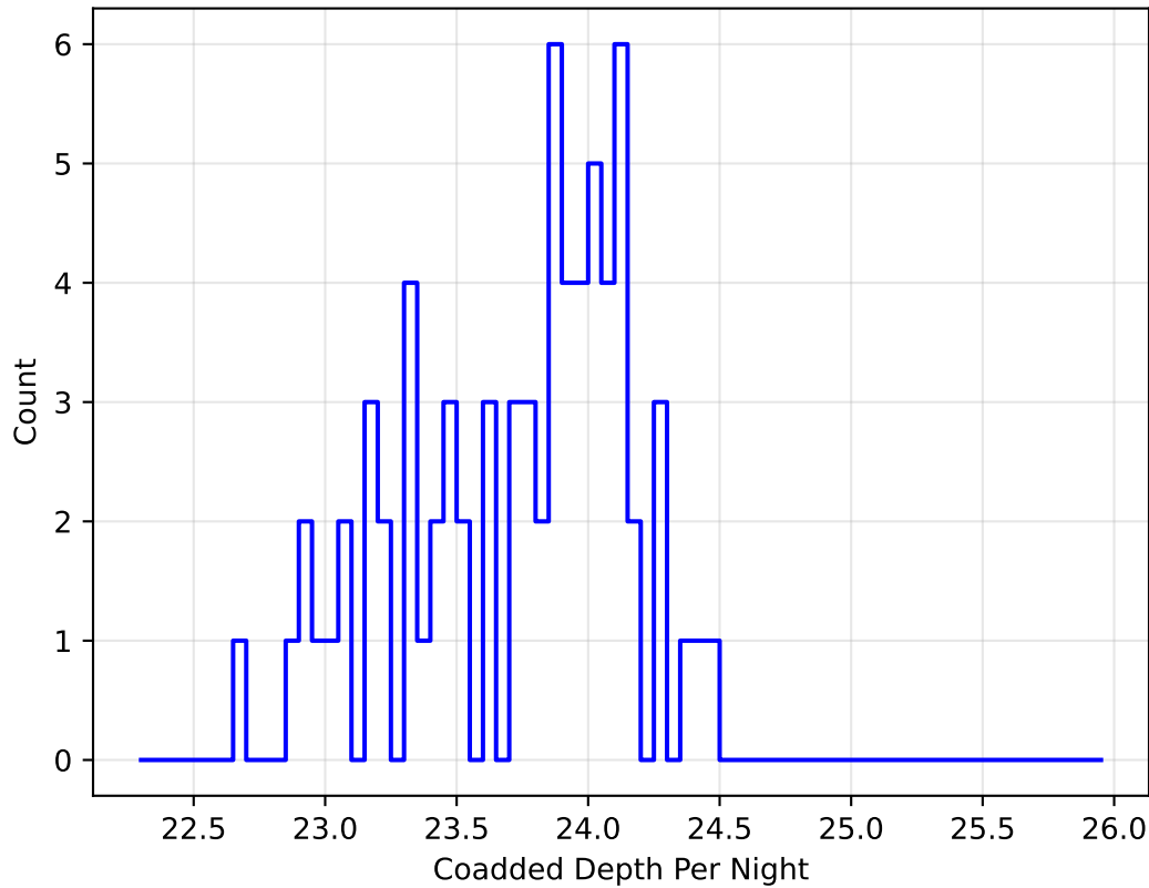
ddf_loaded_half_fl2_v3.4_10yrs u band: DD:XMM_LSS CoaddM5PerNight
