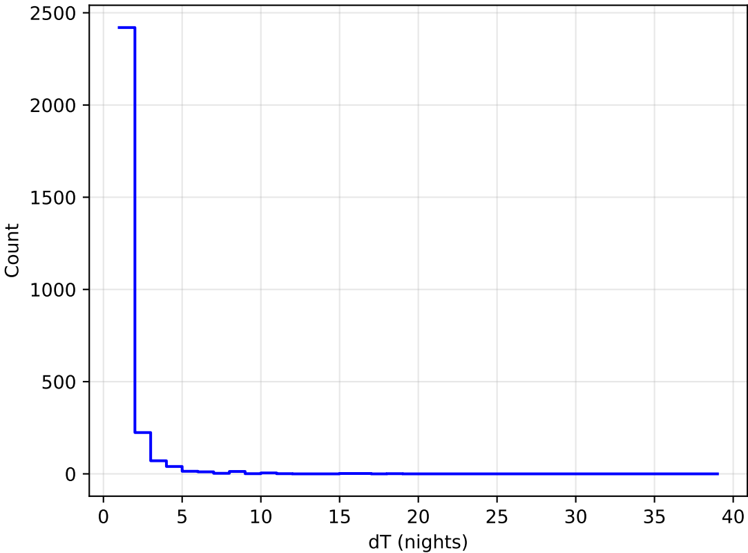
ddf_loaded_half_fl2_v3.4_10yrs all bands: DD:WFD Delta Nights Histogram
