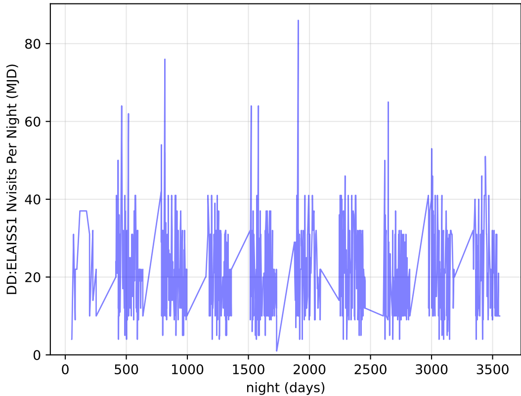
ddf_loaded_half_fl2_v3.4_10yrs all bands: DD:ELAISS1 Nvisits Per Night
