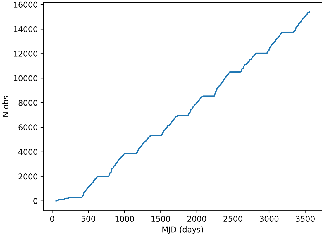
ddf_loaded_half_fl2_v3.4_10yrs all bands: DD:ELAISS1 Cumulative NVisits
