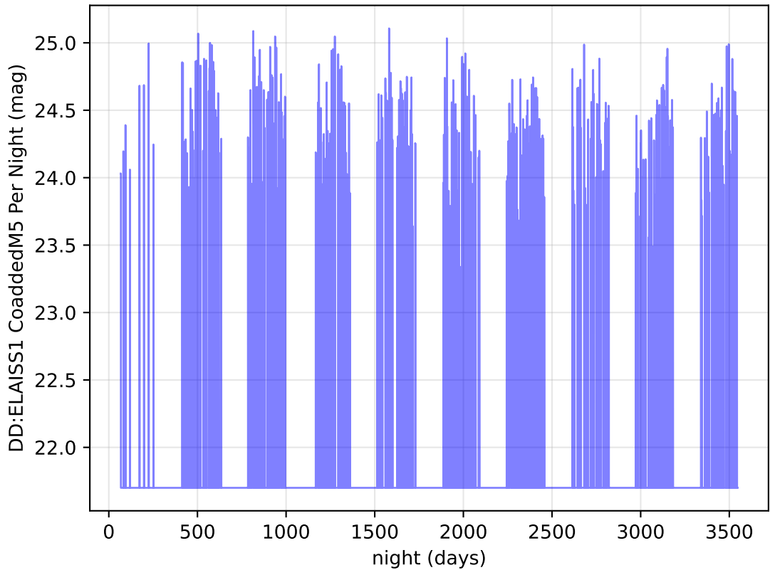
ddf_loaded_half_fl2_v3.4_10yrs z band: DD:ELAISS1 CoaddedM5 Per Night
