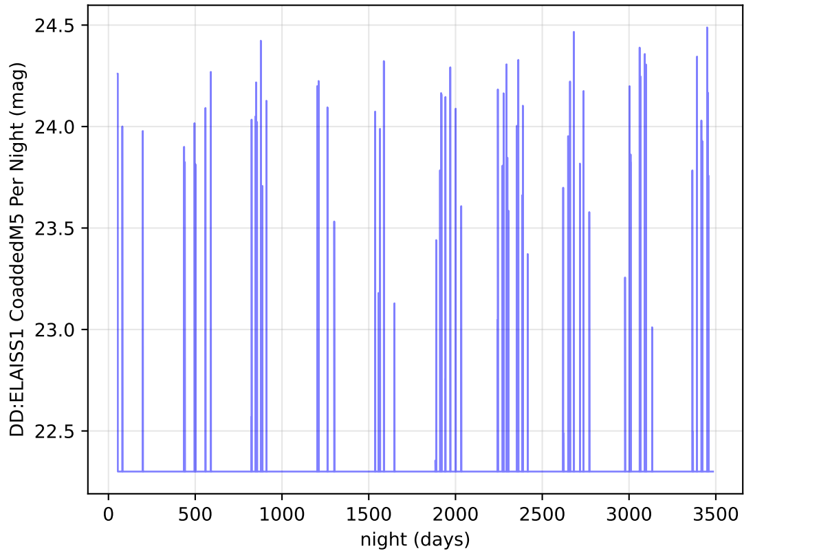
ddf_loaded_half_fl2_v3.4_10yrs u band: DD:ELAISS1 CoaddedM5 Per Night
