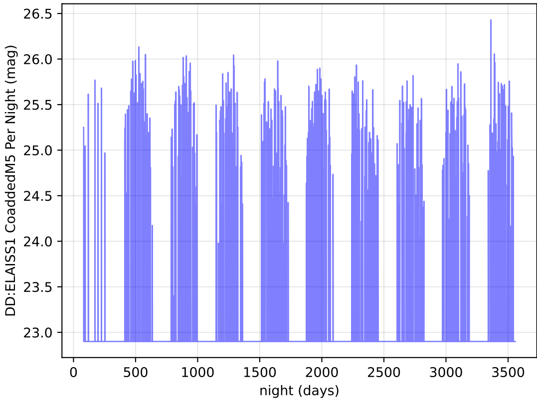
ddf_loaded_half_fl2_v3.4_10yrs r band: DD:ELAISS1 CoaddedM5 Per Night
