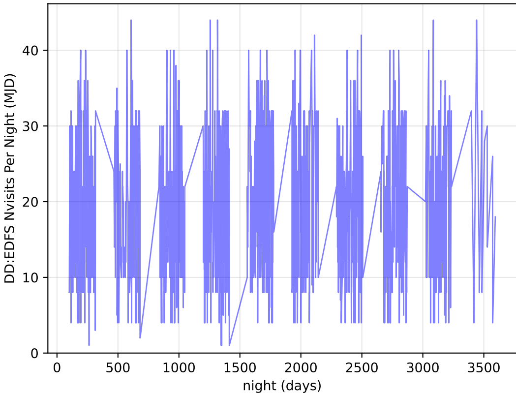
ddf_loaded_half_fl2_v3.4_10yrs all bands: DD:EDFS Nvisits Per Night
