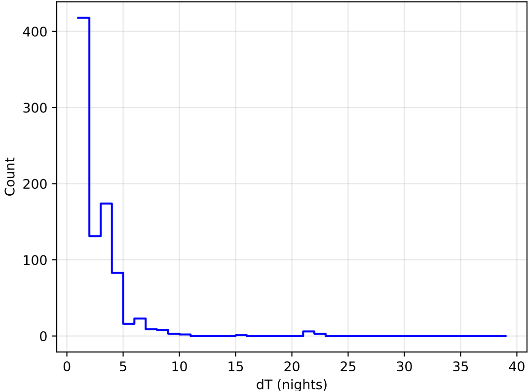
ddf_loaded_half_fl2_v3.4_10yrs all bands: DD:EDFS Delta Nights Histogram
